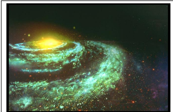
Fig.11 Approaching the Milky Way. ©Jon Lomberg https://www.jonlomberg.com/limited_edition/le_a_approaching_milkyway.html
